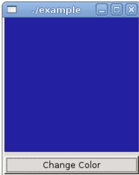
Figure 4-2. Stage Widget
