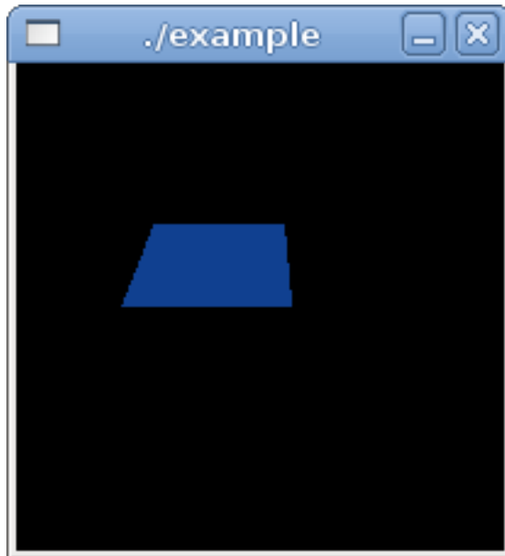
Figure 6-2. Score
