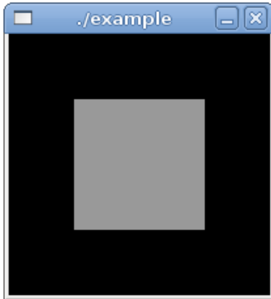
Figure 5-4. Actor Events
